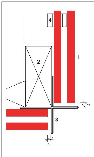
Kreuzeckprofil, Steg 29 mm
