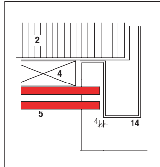
Fensterzarge
